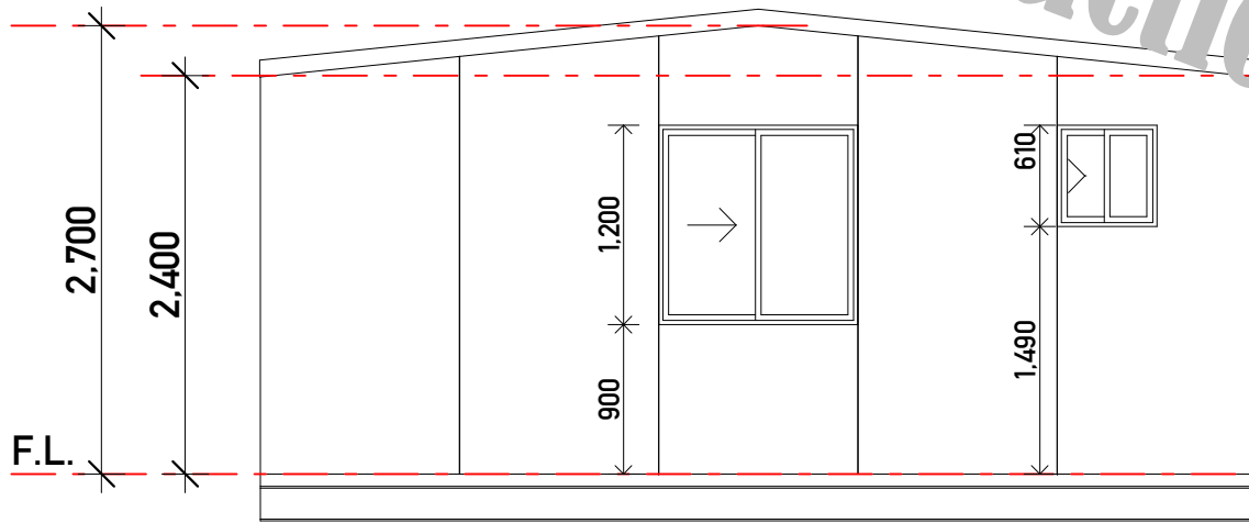
Elevation C Scale 1:50
