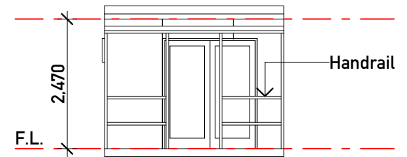
Elevation D Scale 1:100
