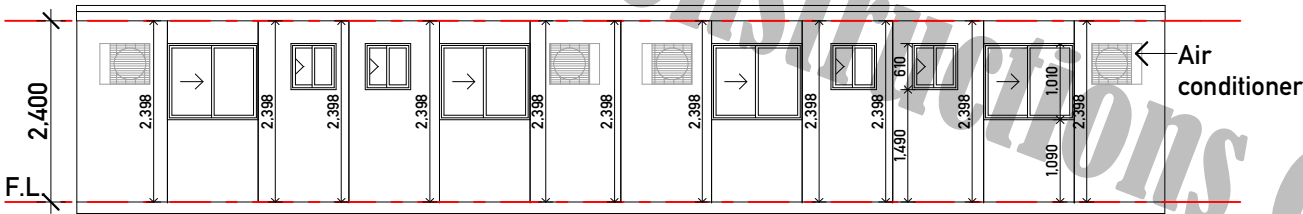
Elevation C Scale 1:100
