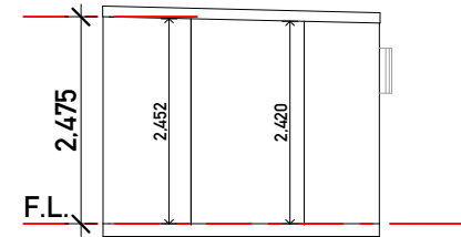
Elevation D Scale 1:100
